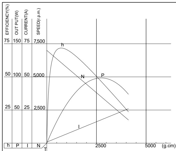
RS775SM-6027-97 12.0V
