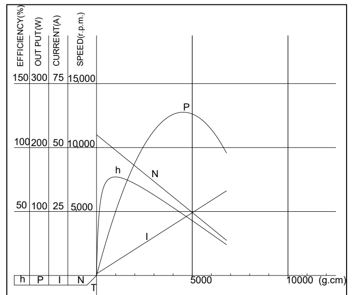
RS775SM-5035-97 24.0V
