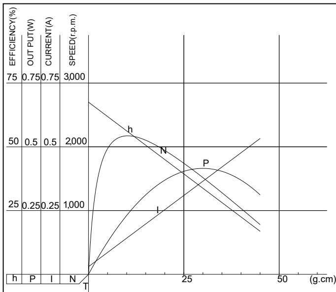
RE500CP-18280-33 3.0 V
